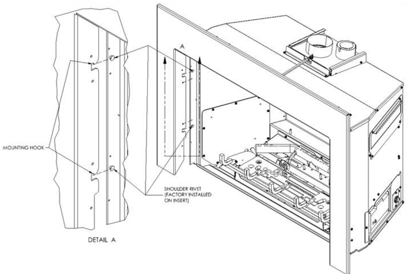
Surround Installation
