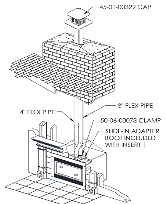
Vent System
