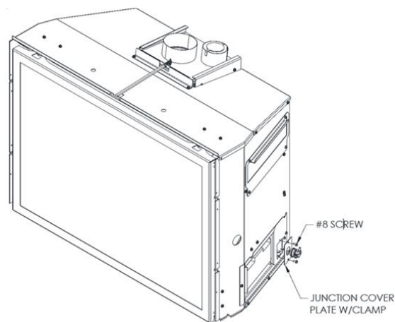
Electrical Junction Box
