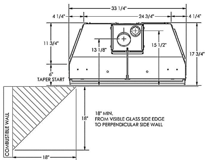
Side Wall Clearances
