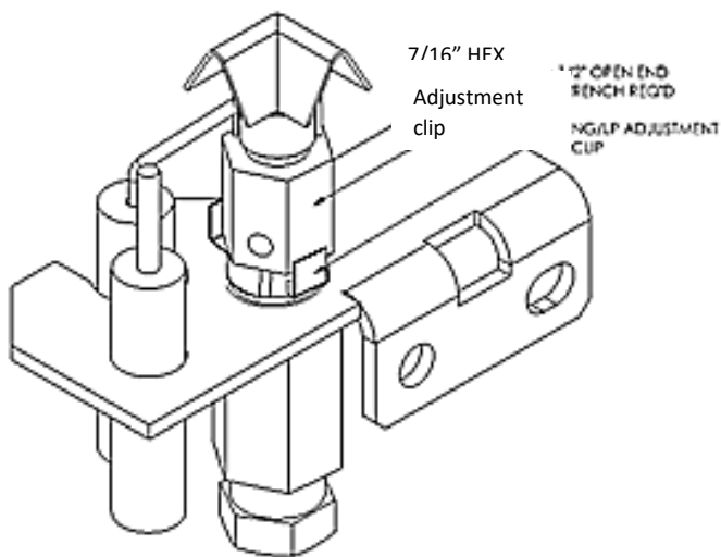
Pilot Body
