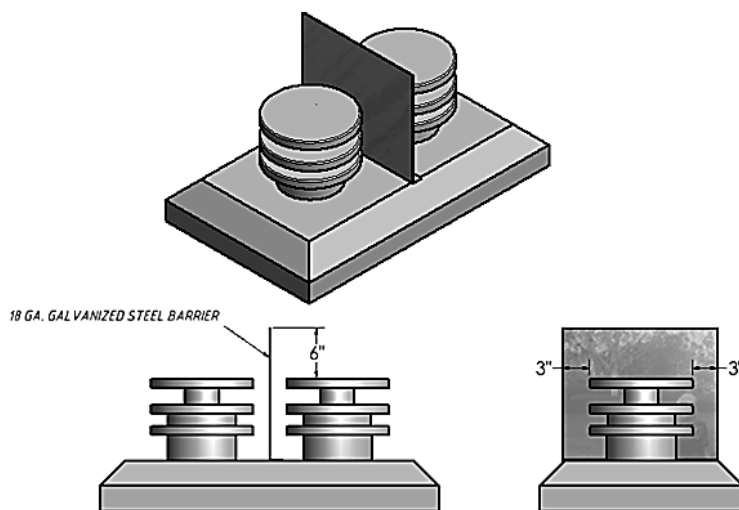
Side by Side Vent Caps
