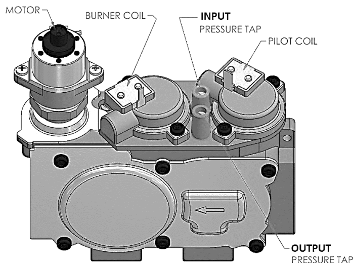
Main Gas Valve
