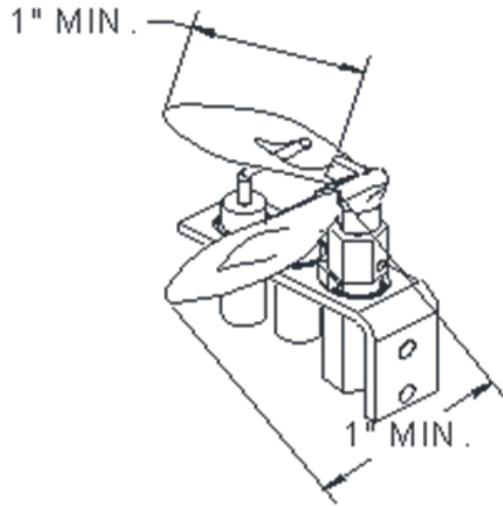
Minimum Pilot Flame Length
