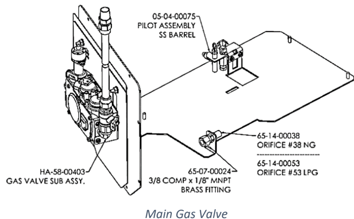
Main Gas Valve
